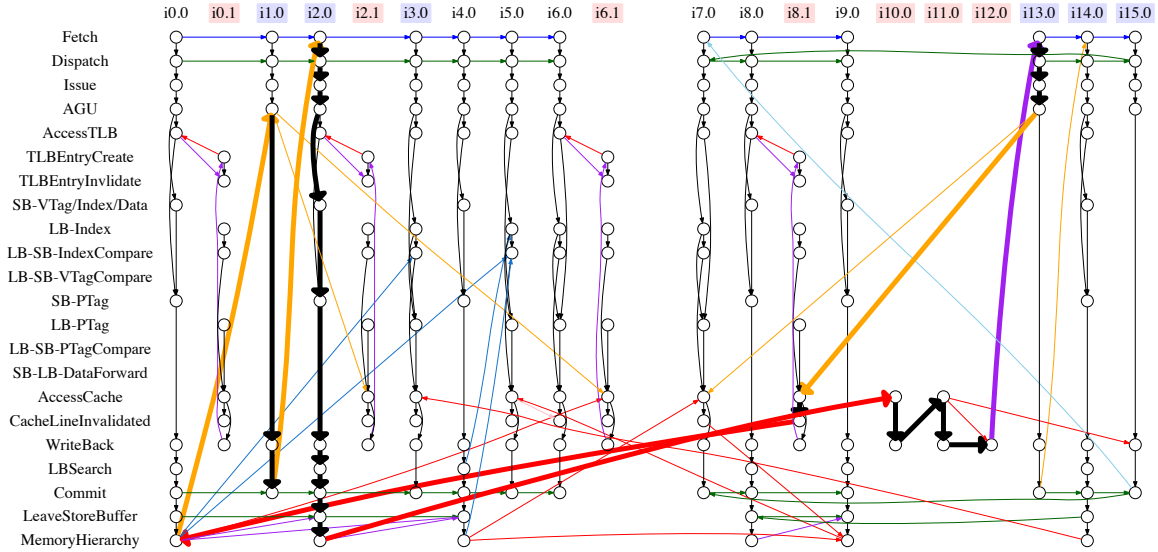
Figure 11: Cyclic graph illustrating one possible ordering for litmus test ipi8 [38, 39]. Because the graph is cyclic (highlighted with thicker edges), this outcome is not observable in this case. In this case, the cycle was found before the PTEs for y were even enumerated. For this test, all executions lead to cyclic graphs, and hence the outcome is not observable, as expected.
