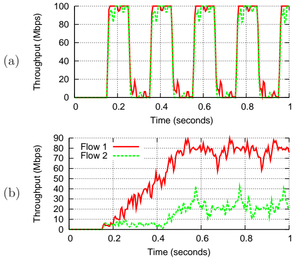
Figure 3: (a) Simulation demonstrating oscillatory behavior in the example of Fig. 1. (b) The same scenario with different initial conditions.
