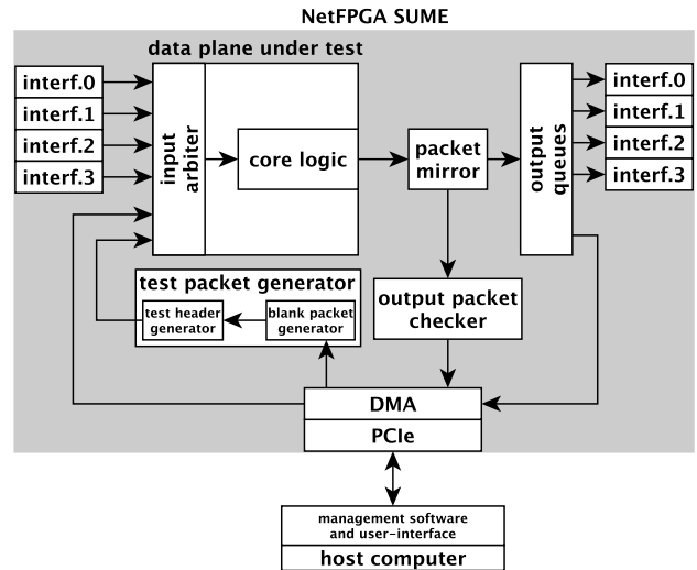
Figure 5: NetFPGA SUME implementation.
