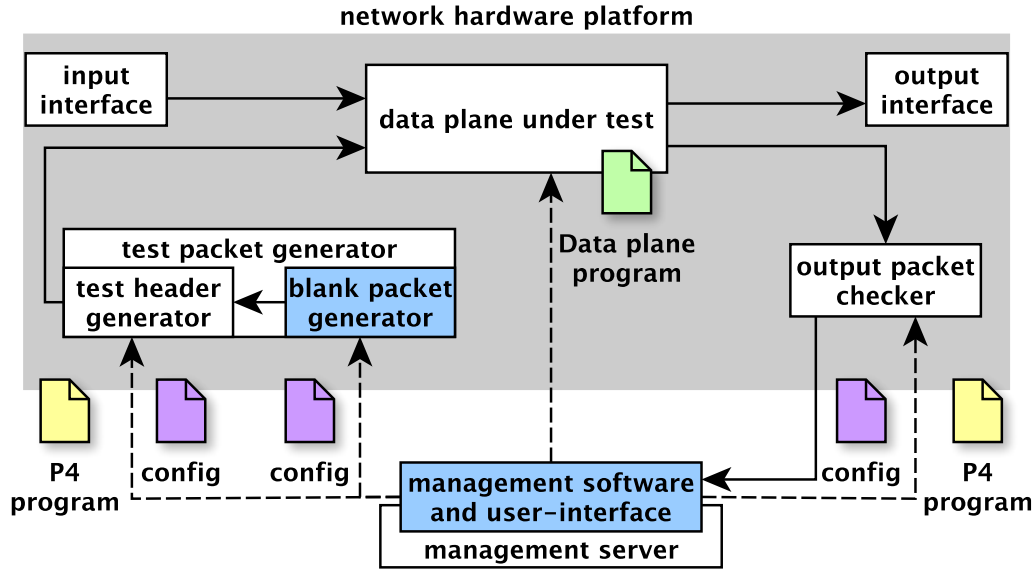
Figure 1: The proposed architecture: target specific infrastructure (light-blue), portable suite of P4 test programs (yellow) and test-specific configurations (purple).
