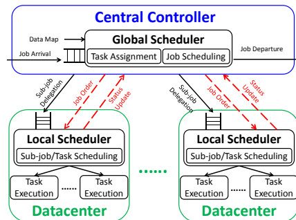
Figure 1. System Architecture of Distributed Job Execution
