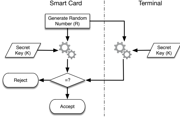
Fig. 5: External authentication, used by the card to validate the terminal.
