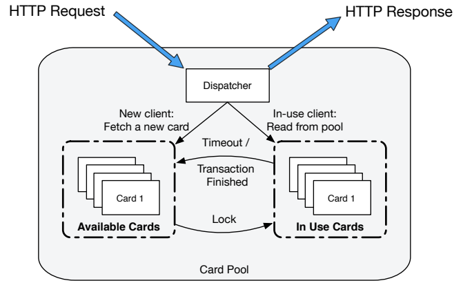
Fig. 7: Card pool scheduler.
