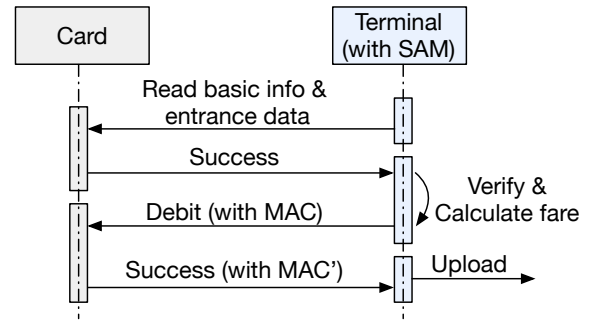
Fig. 4: The exit protocol.
