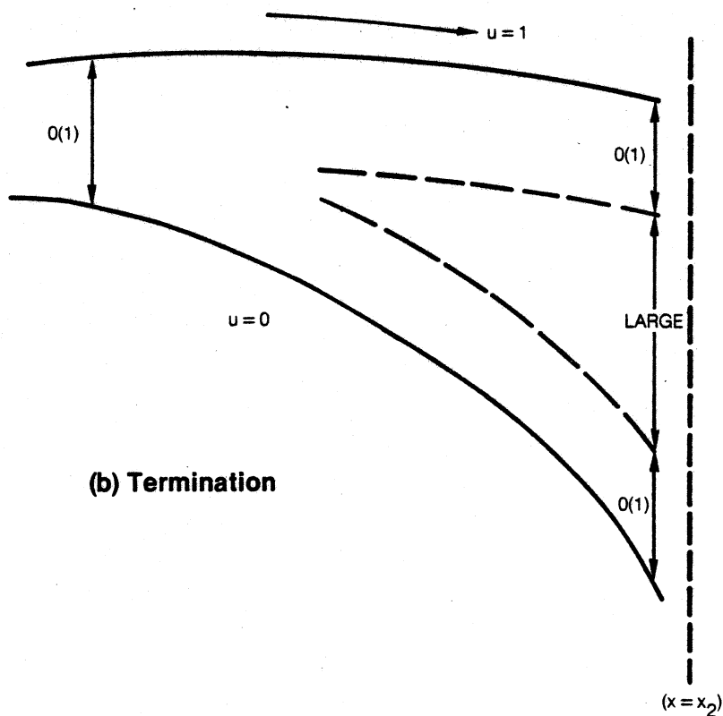
Figure 12 Non-entraining Shear Layer Structure
