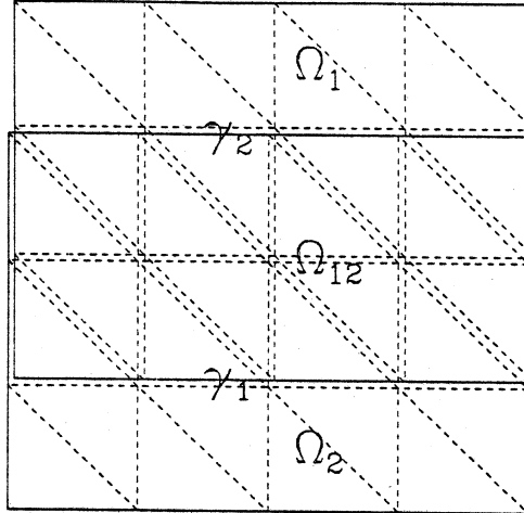
Figure 6: Sample domain illustrating the overlap decomposition (subdomains staggered for clarity).
