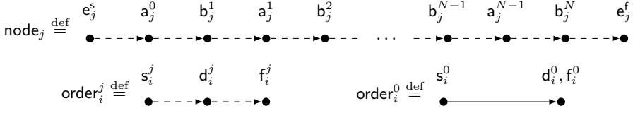
Fig. 2. Graphical representation of the formulas \text{node}_i^j and \text{order}_i^j
