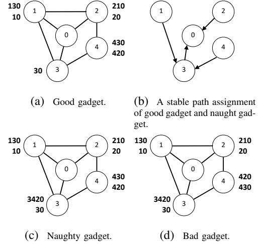
Fig. 1: Examples of stable path problems taken from [1].
