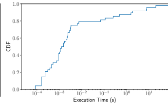
(c) CDF of the time GREEDYMIS uses to find a stable path solution.
