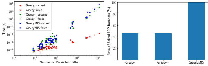
(a) Detailed solvability and execution time of GREEDYMIS. (b) Percentage of SPP instances different algorithms solved.
