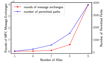
Fig. 7: Rounds of communications performed by P-GREEDYMIS protocol.
