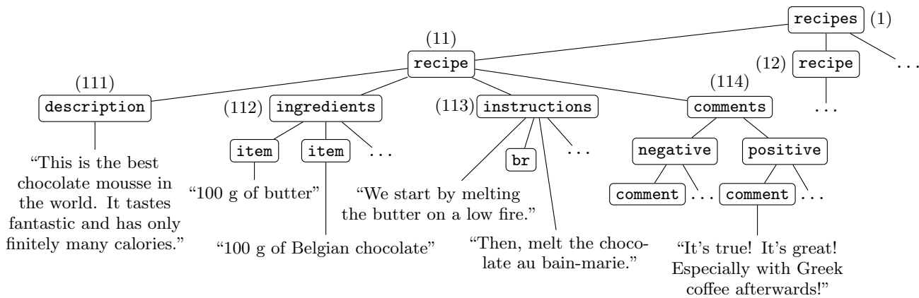
Figure 1: A text tree representing an XML document for recipes.
